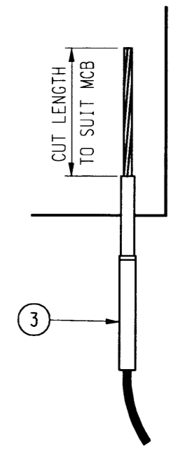
DETAIL 2
