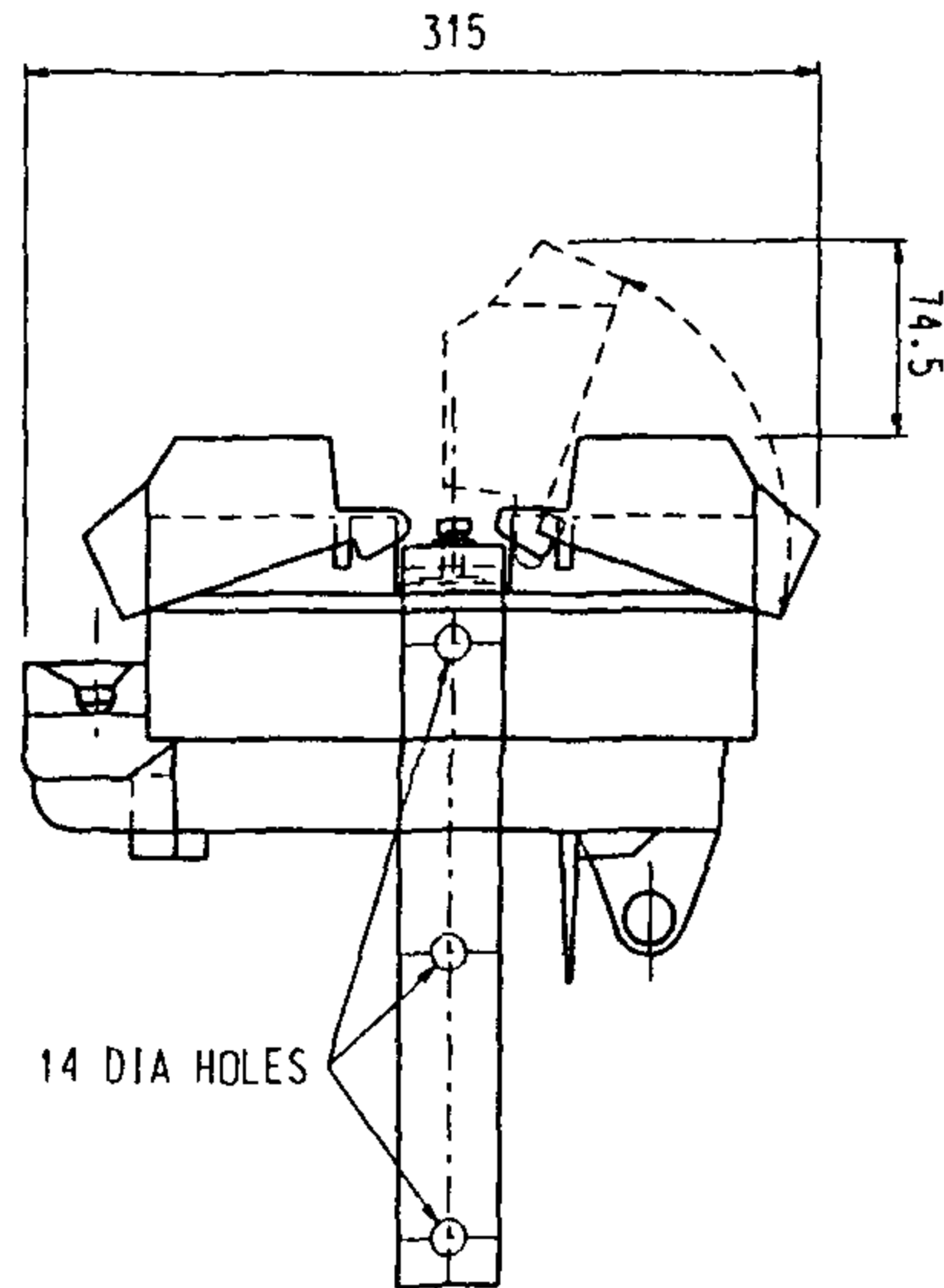
ITEM 1 SWITCH LV COMBINATION ISOLATOR/FUSE 250 A
