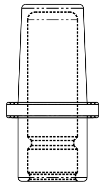
DETAIL A - ABC CABLE SEAL (95-150mm) ITEM NUMBER 504107
