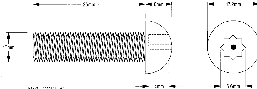
M10 SCREW STOCK CODE 402032
