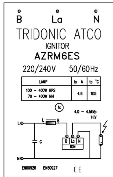
IGNITOR WIRING CIRCUIT DETAIL
