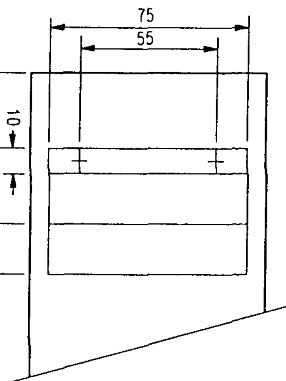
MOUNTING DETAIL
