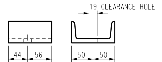
DETAIL B 1:5
