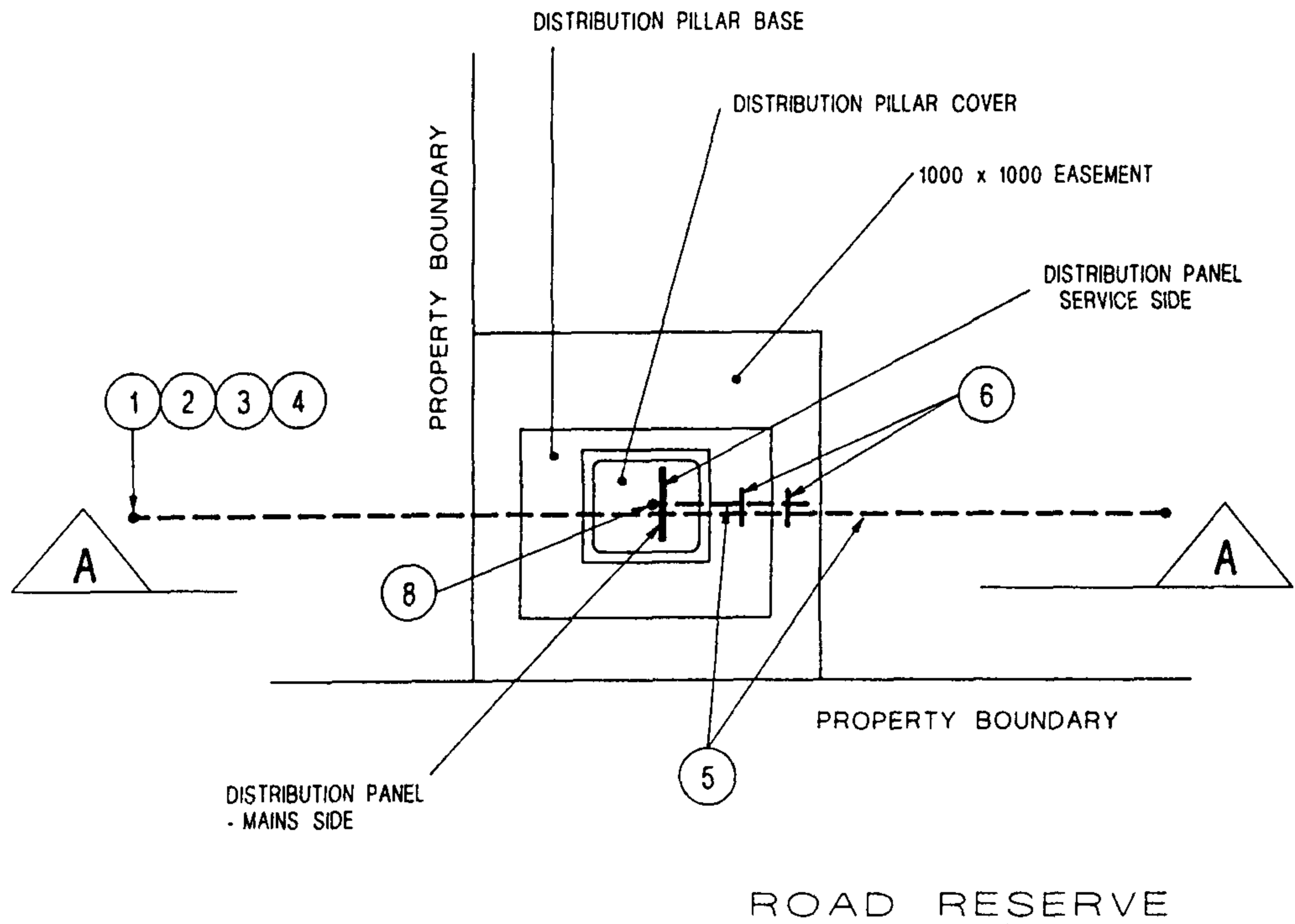
PLAN
