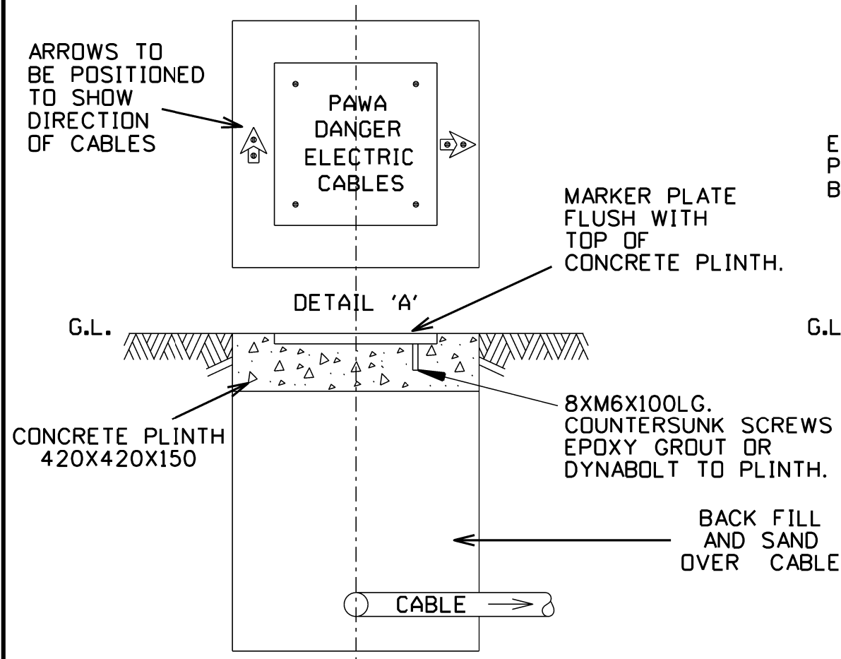
TYPICAL INSTALLATION CABLE ROUTE MARKER STOCK CODE 5066
