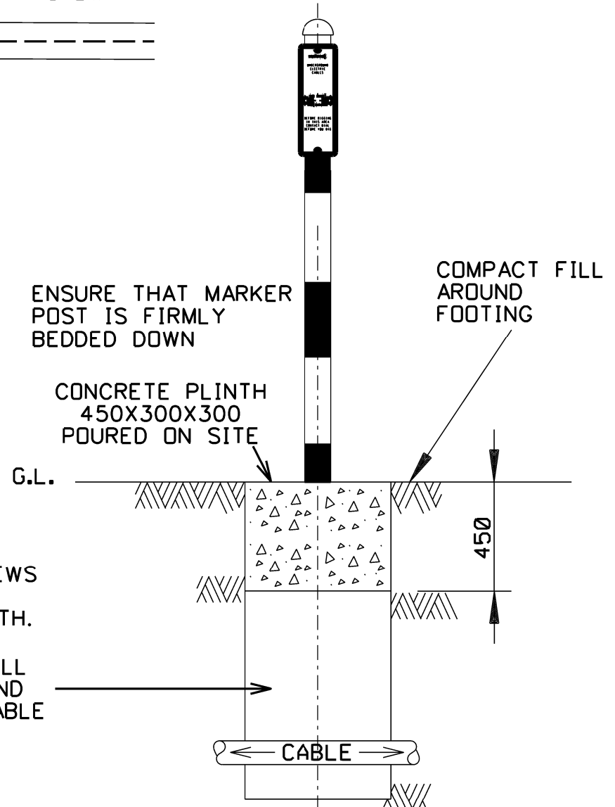
TYPICAL INSTALLATION CABLE ROUTE MARKER STOCK CODE 11007
