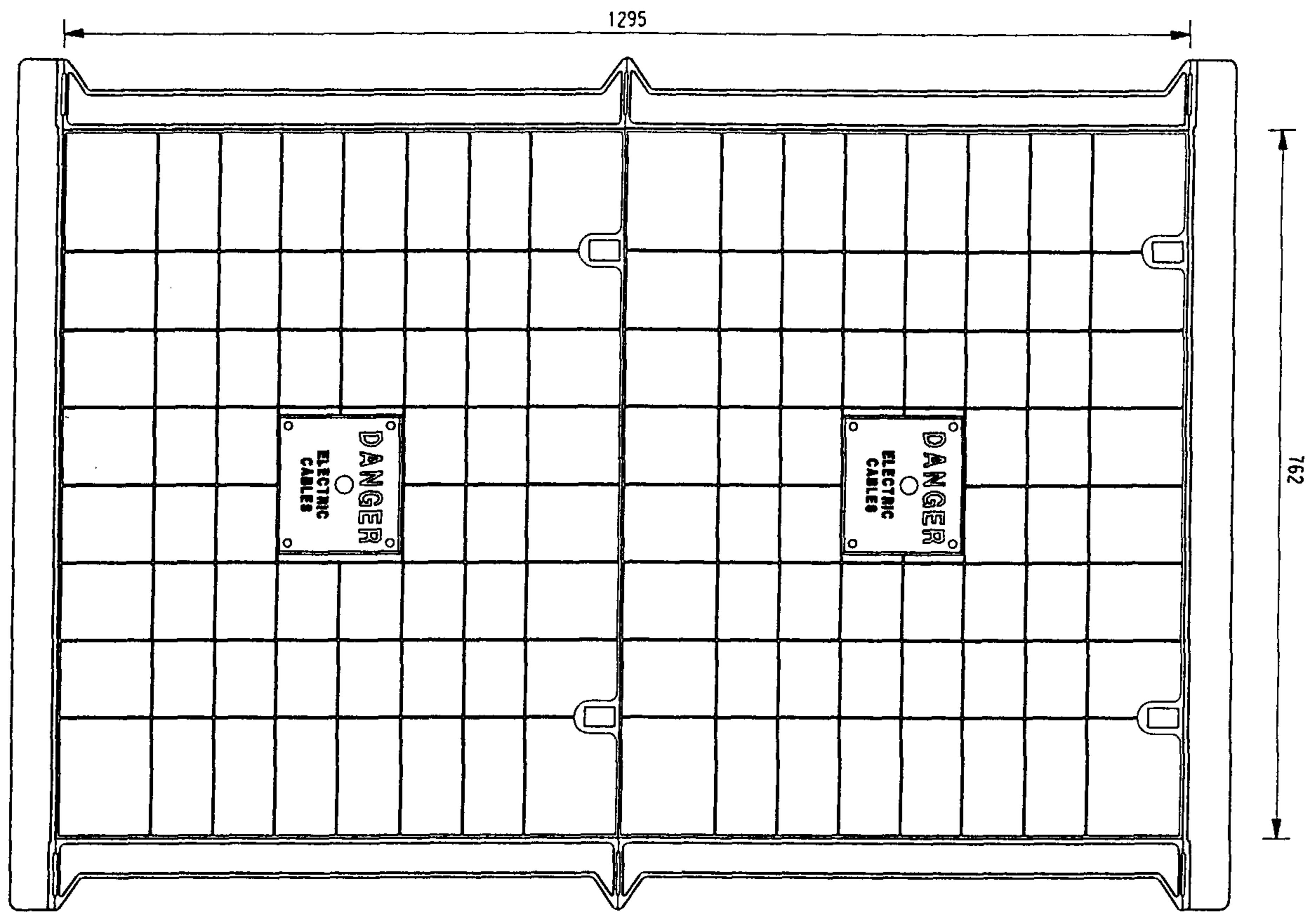
ITEM 1 : ACCESS COVER AND FRAME, 2 PART COVER, CLASS 'D' (STOCK CODE : 8805)
