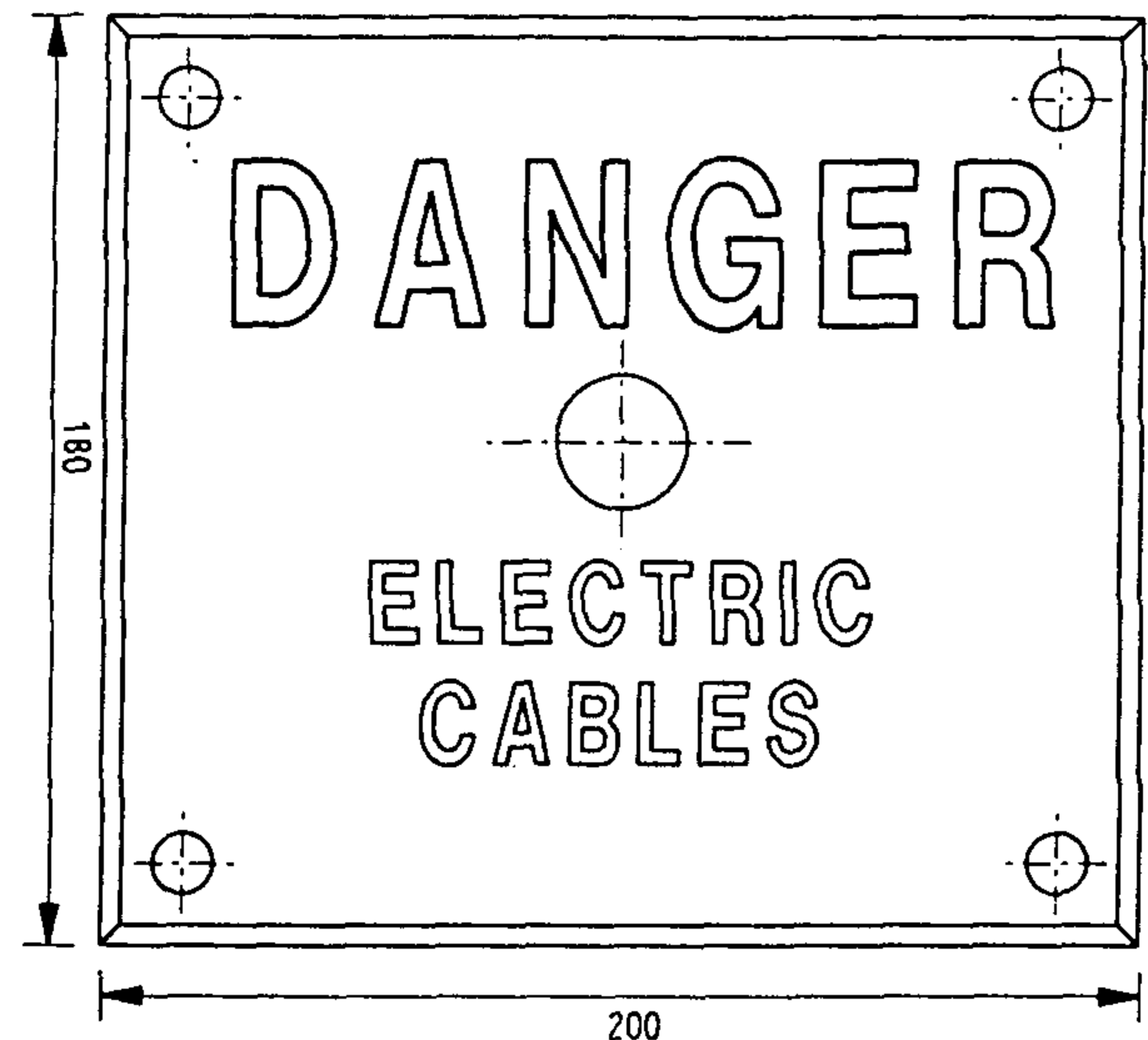
ITEM 2 : ACCESS COVER MARKER PLATE (STOCK CODE : 7625)
