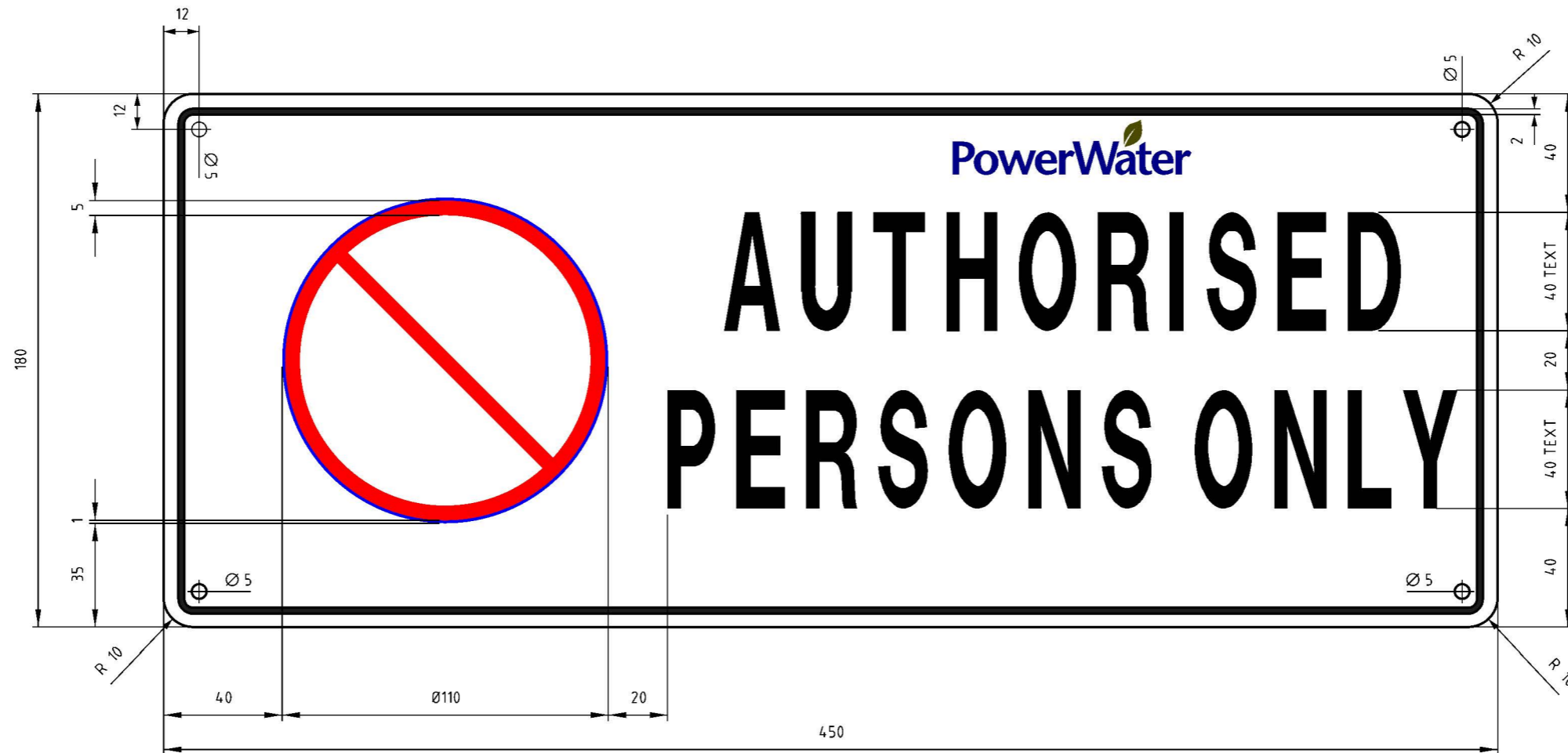
PLAN LAYOUT
