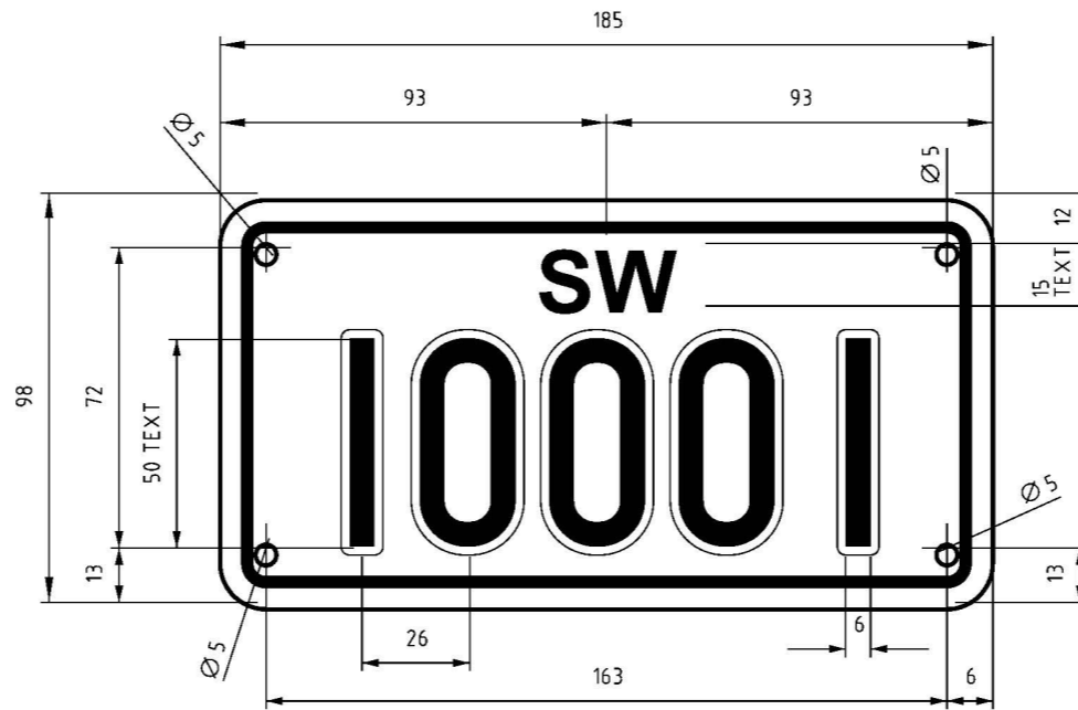
DISTRIBUTION SWITCHGEAR NUMBER PLATE PLAN VIEW SCALE 1:2
