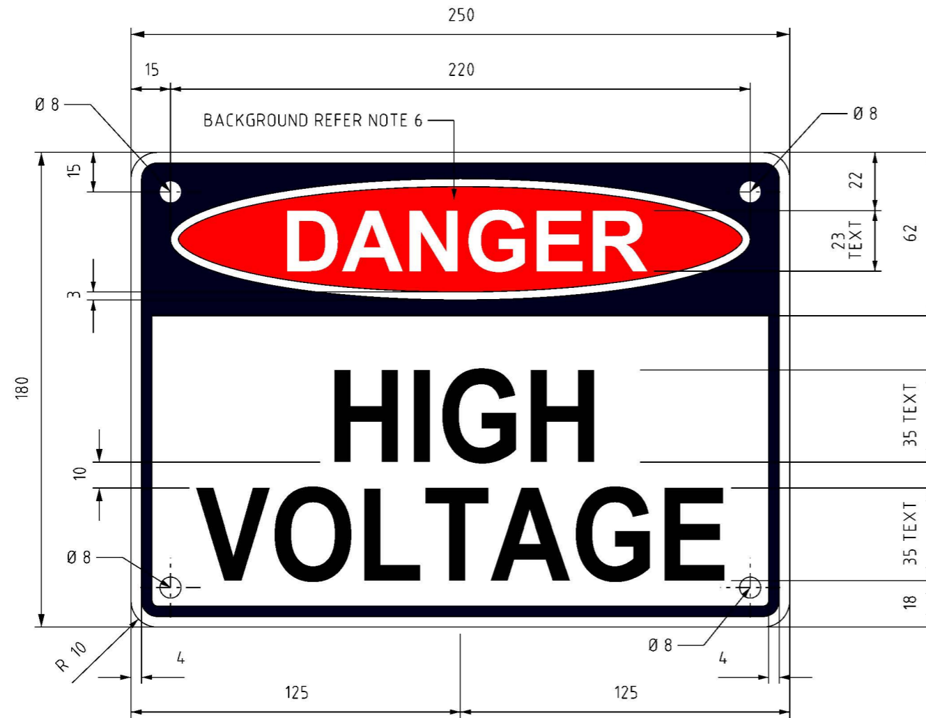
SIGNS DANGER H.V. PLAN VIEW
