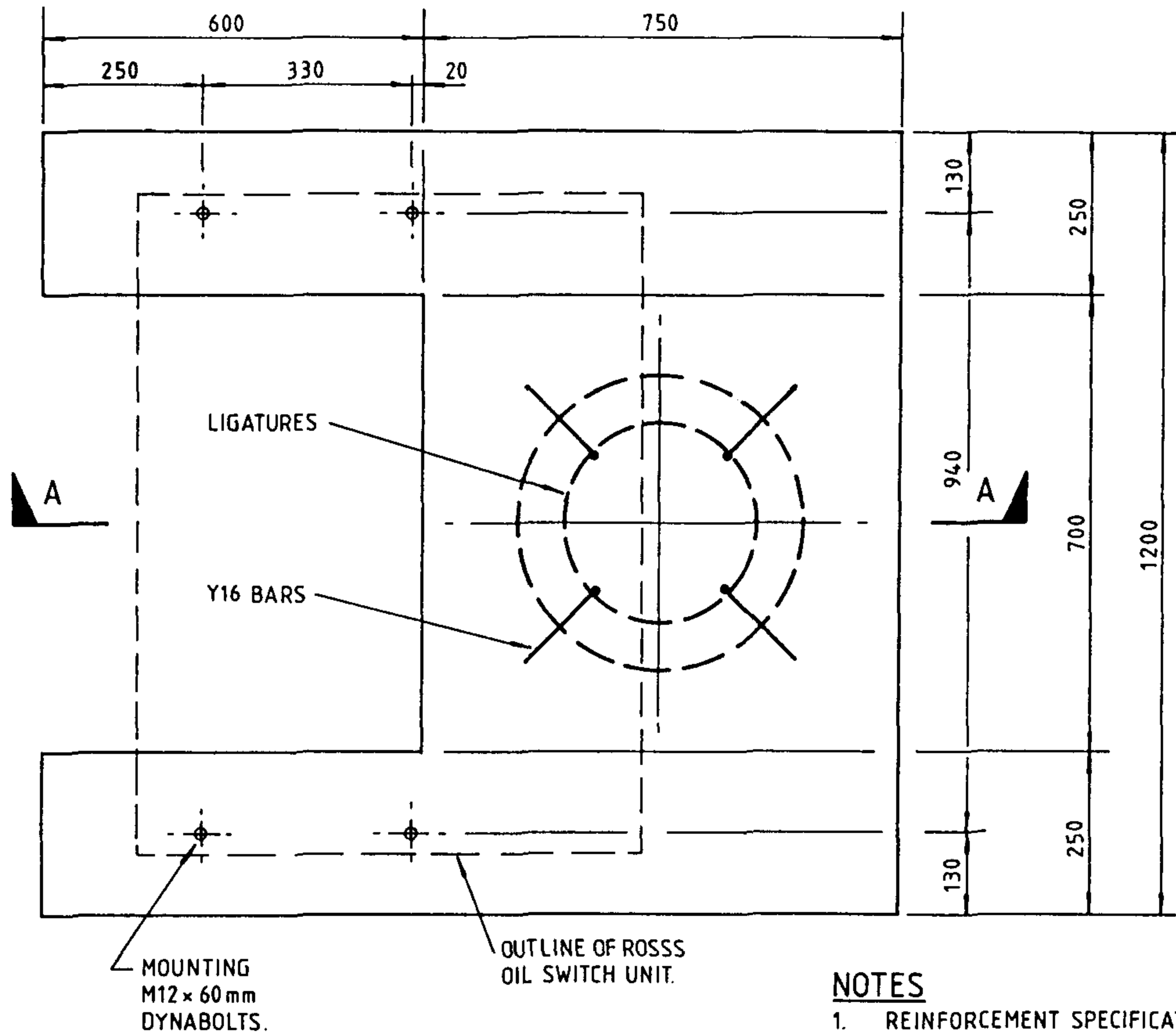
PLAN VIEW (MESH NOT SHOWN)
