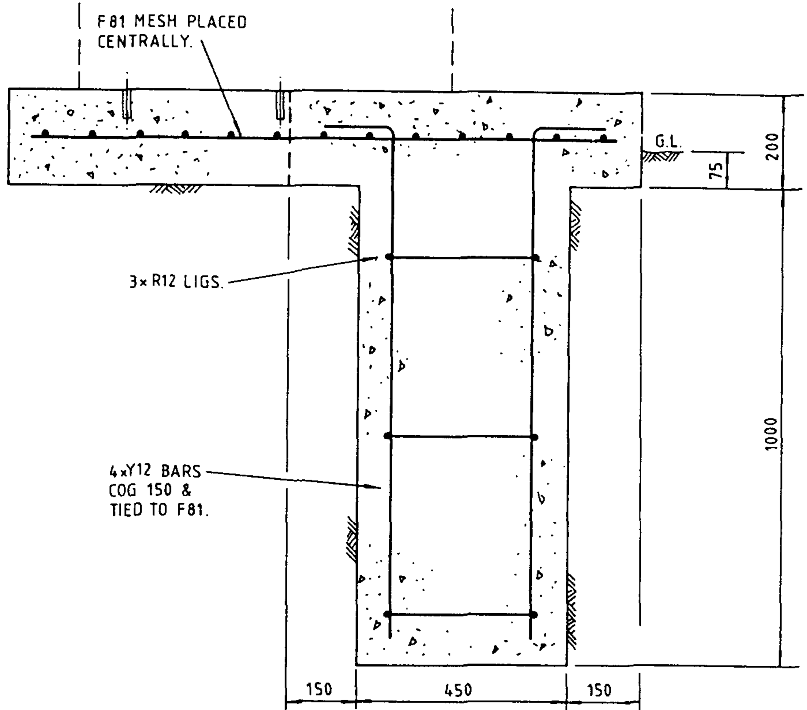
SECTION A - A
