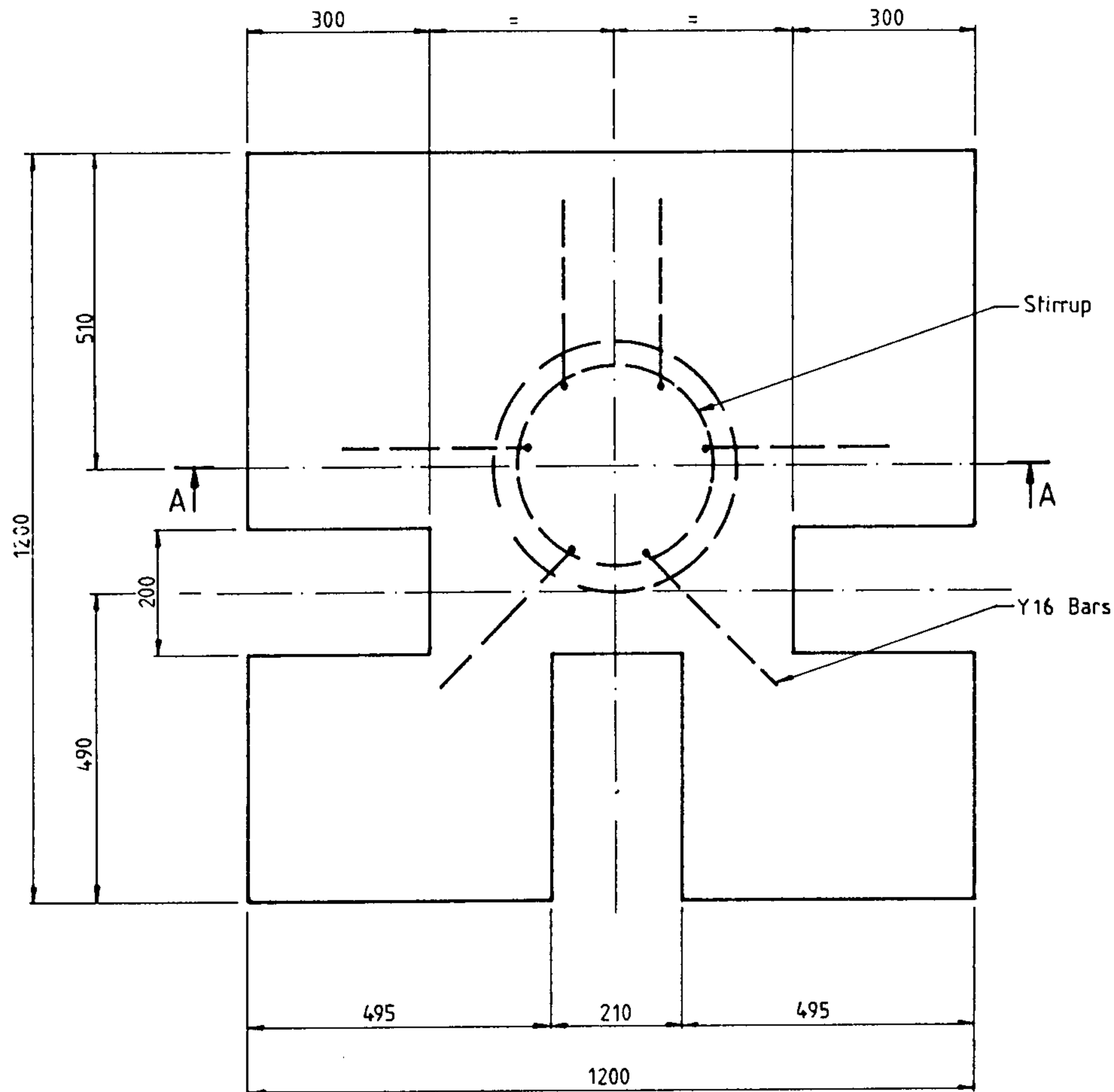
PLAN VIEW (Mesh not shown.)
