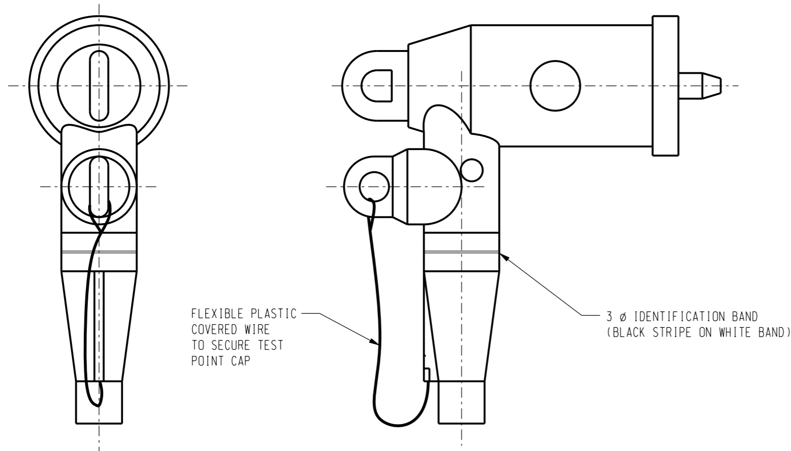
R.T.E. SBT IV WITH TEST POINT ILLUSTRATED
