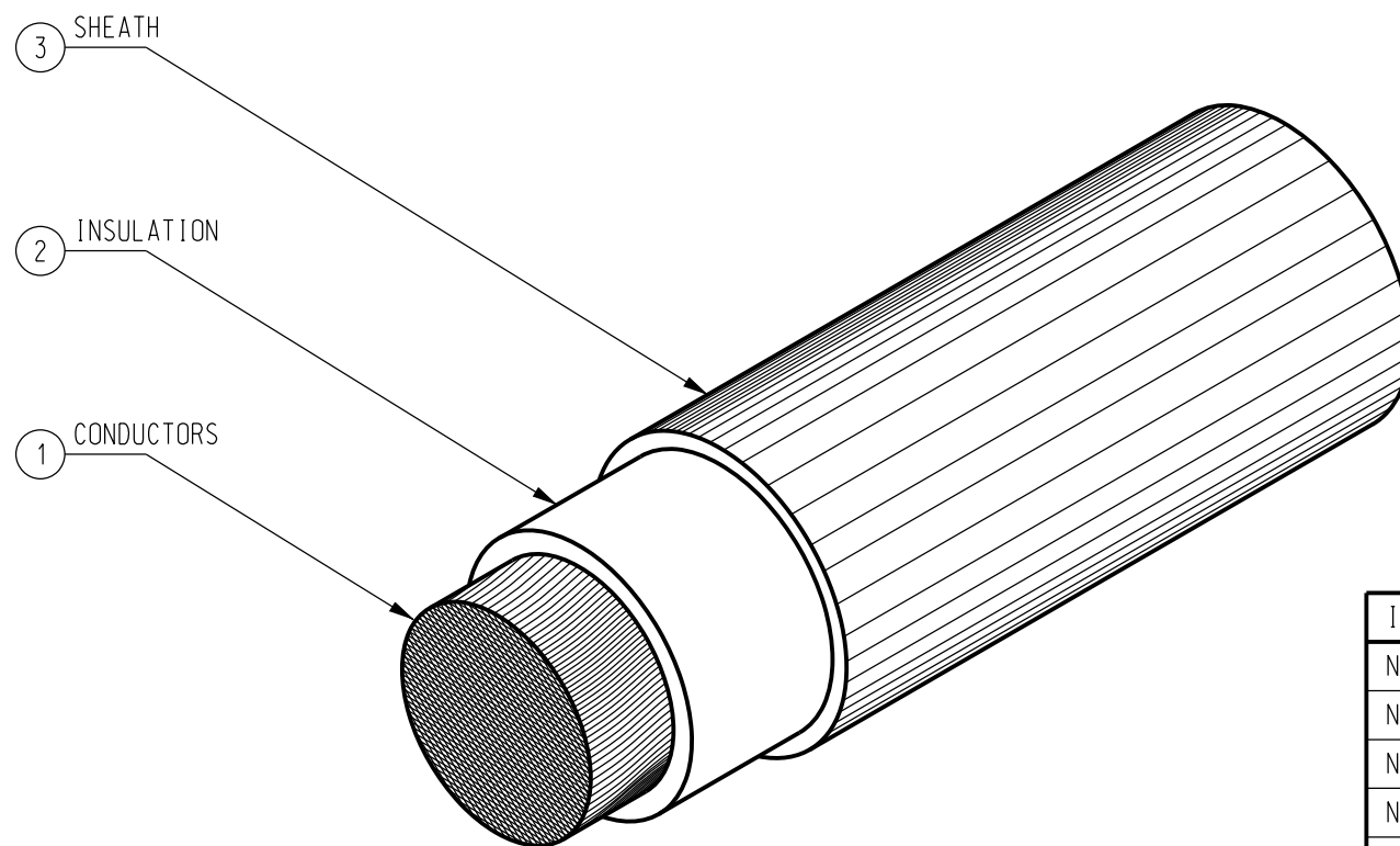
ISOMETRIC VIEW
