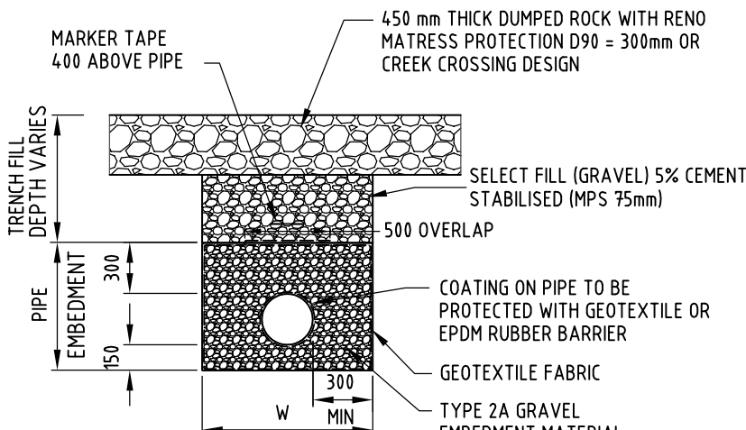
TRENCH DETAIL 5 CREEK CROSSING
