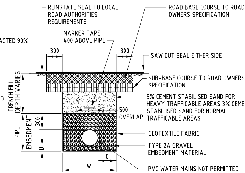
TRENCH DETAIL 3 ROAD CROSSING
