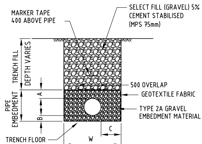
TRENCH DETAIL 4 DRAIN CROSSING
