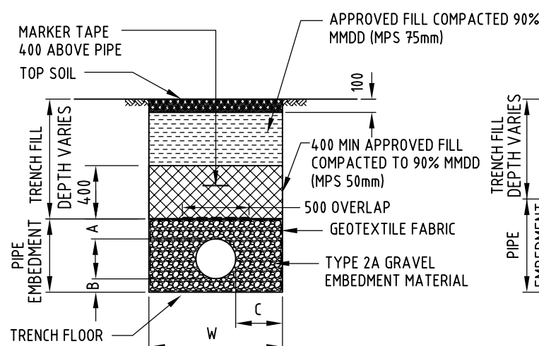
TRENCH DETAIL 2 GENERAL AREA
