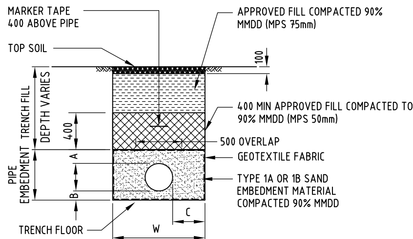
TRENCH DETAIL 1 GENERAL AREA UP TO AND INCLUDING DN300
