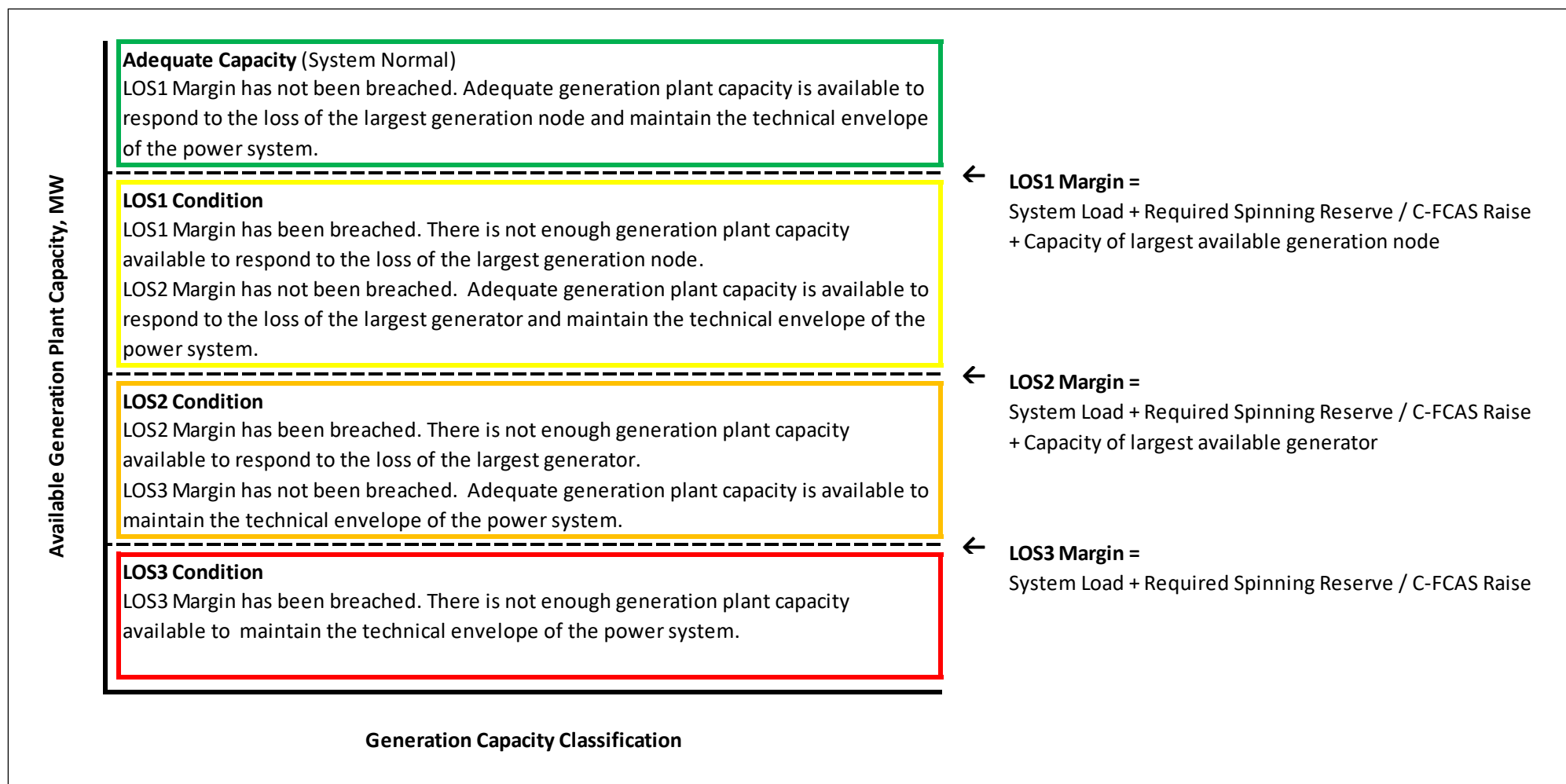
Figure 1: LOS Classification
