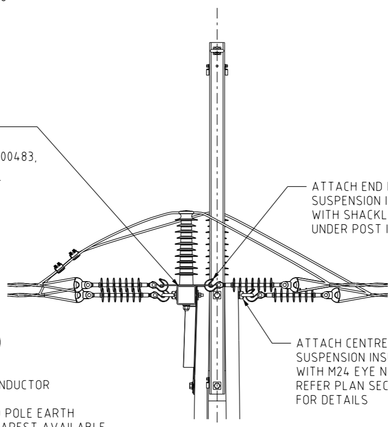
FRONT SIDE SCALE 1:25
