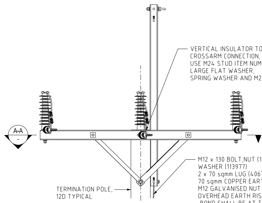
FRONT VIEW SCALE 1:25
