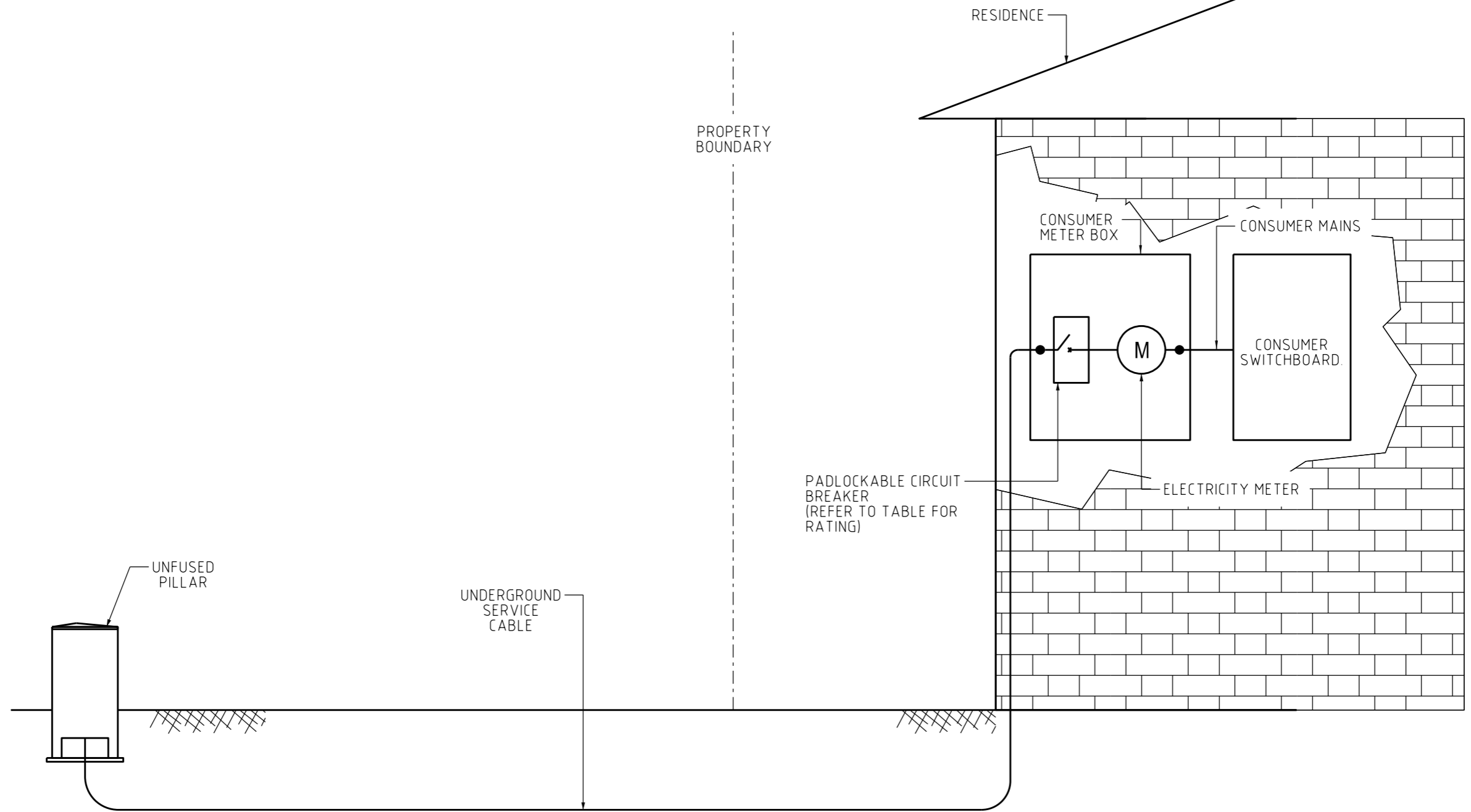
SCENARIO 2 - UNDERGROUND SERVICE CABLE FROM UNFUSED PILLAR AND/OR CONSUMER MAINS CABLE (SINGLE PHASE)
