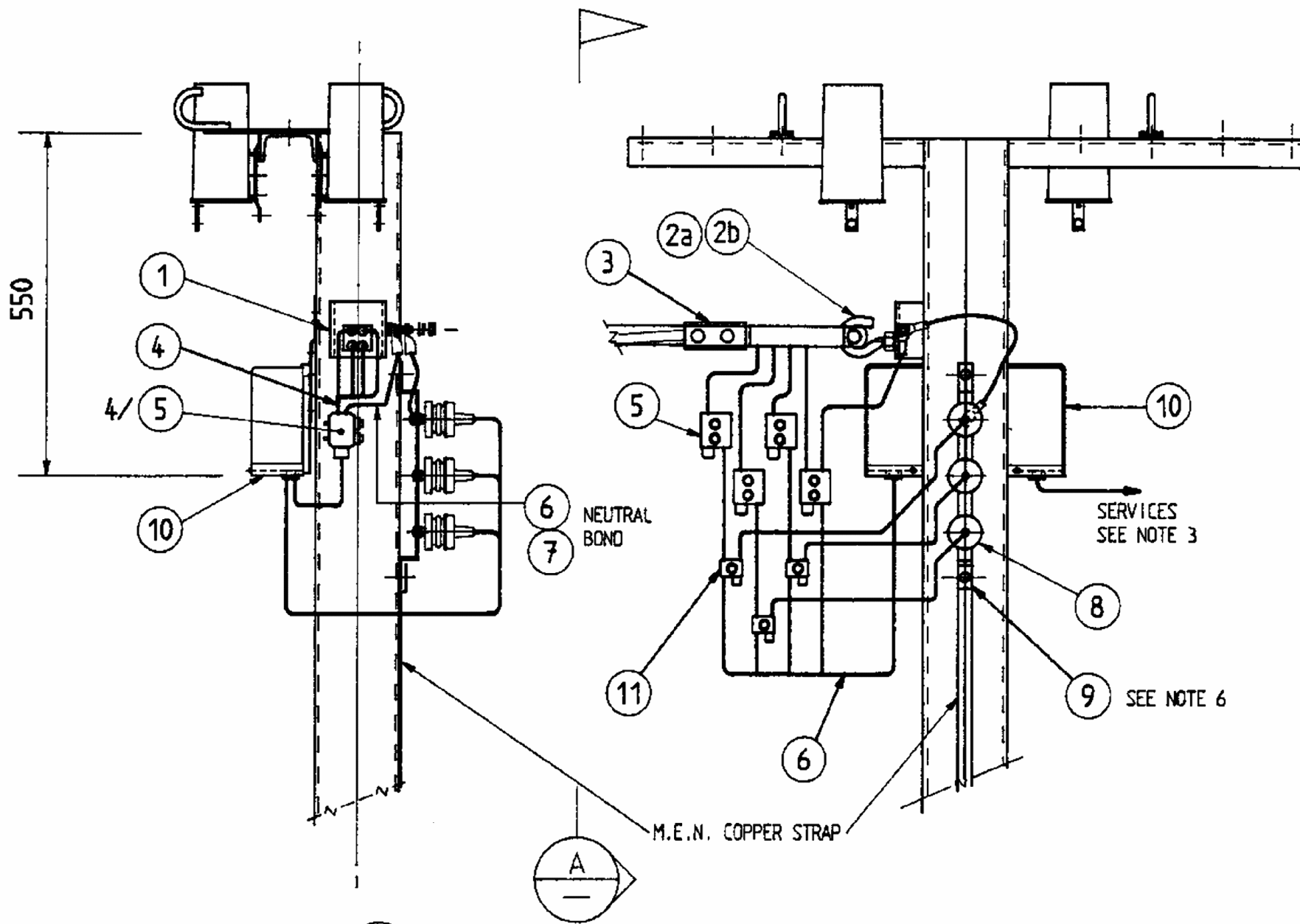
VIEW Scale 1: 10
