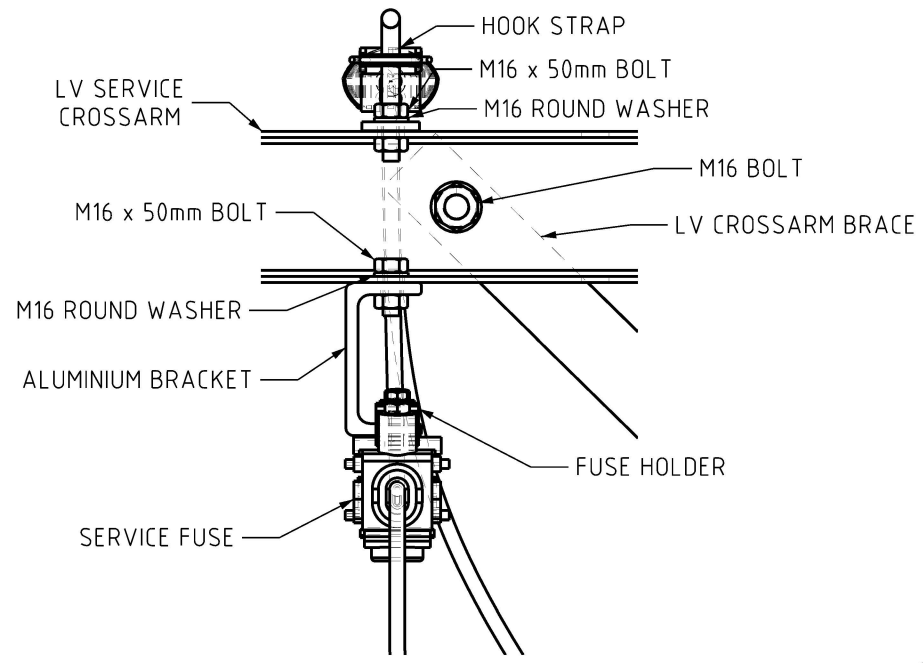
1 DETAIL Sheet-2 1:5
