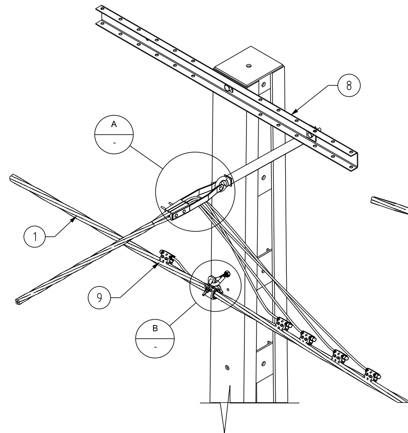
ISOMETRIC FRONT VIEW SCALE N.T.S.
