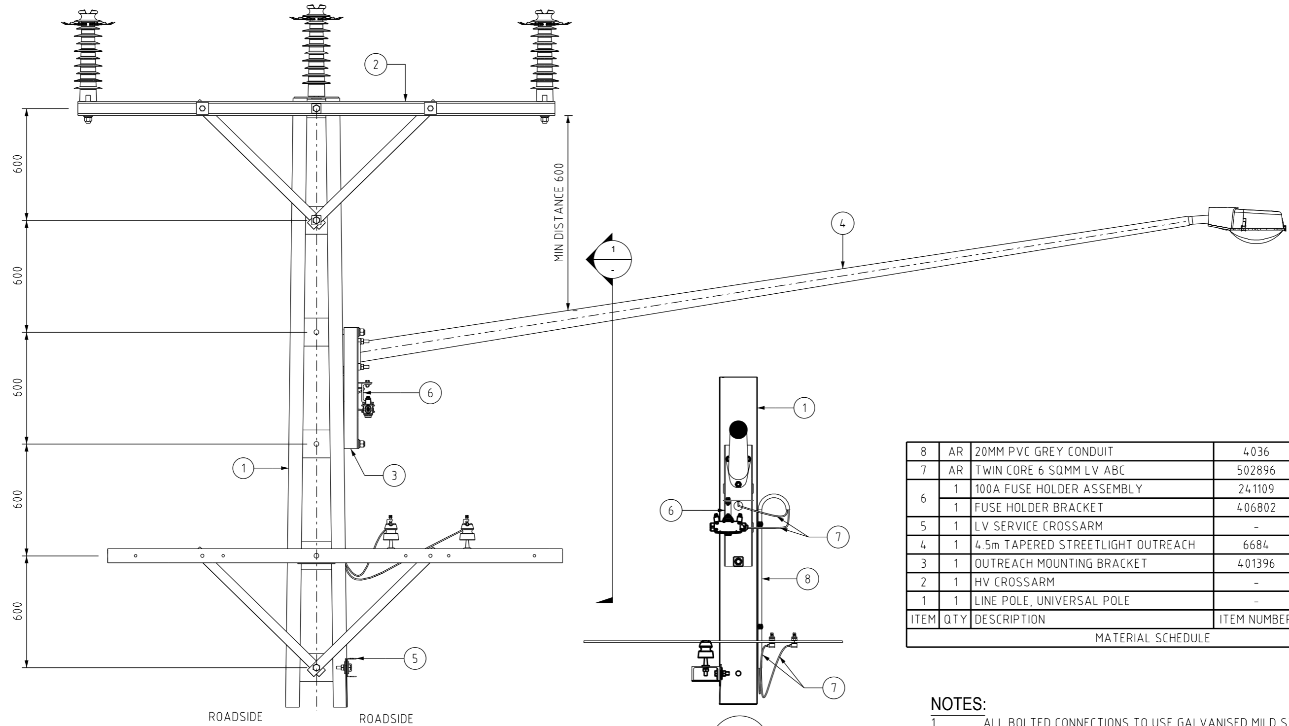
SECTION 1 1:20
