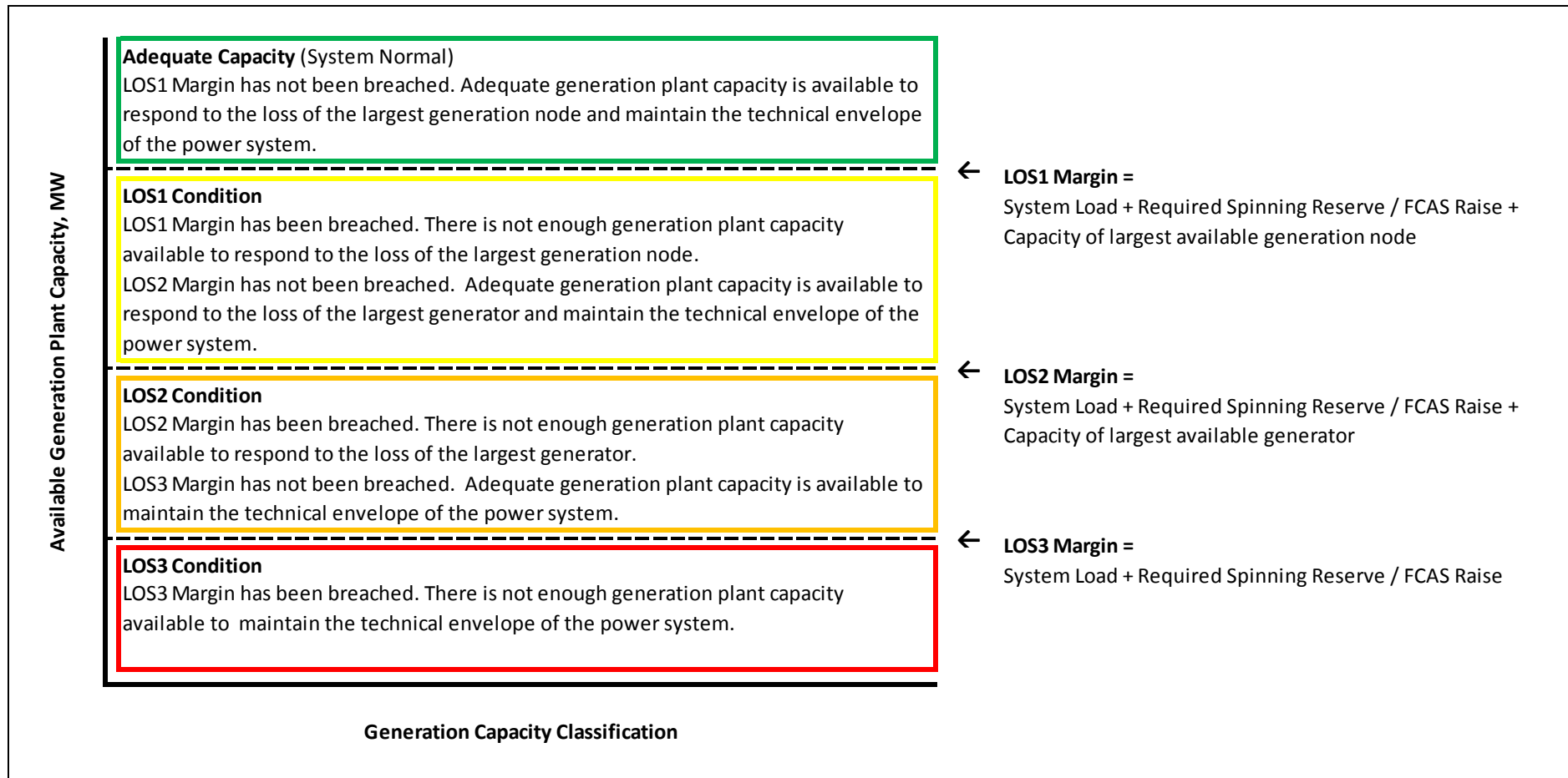
Figure 1: LOS Classification
