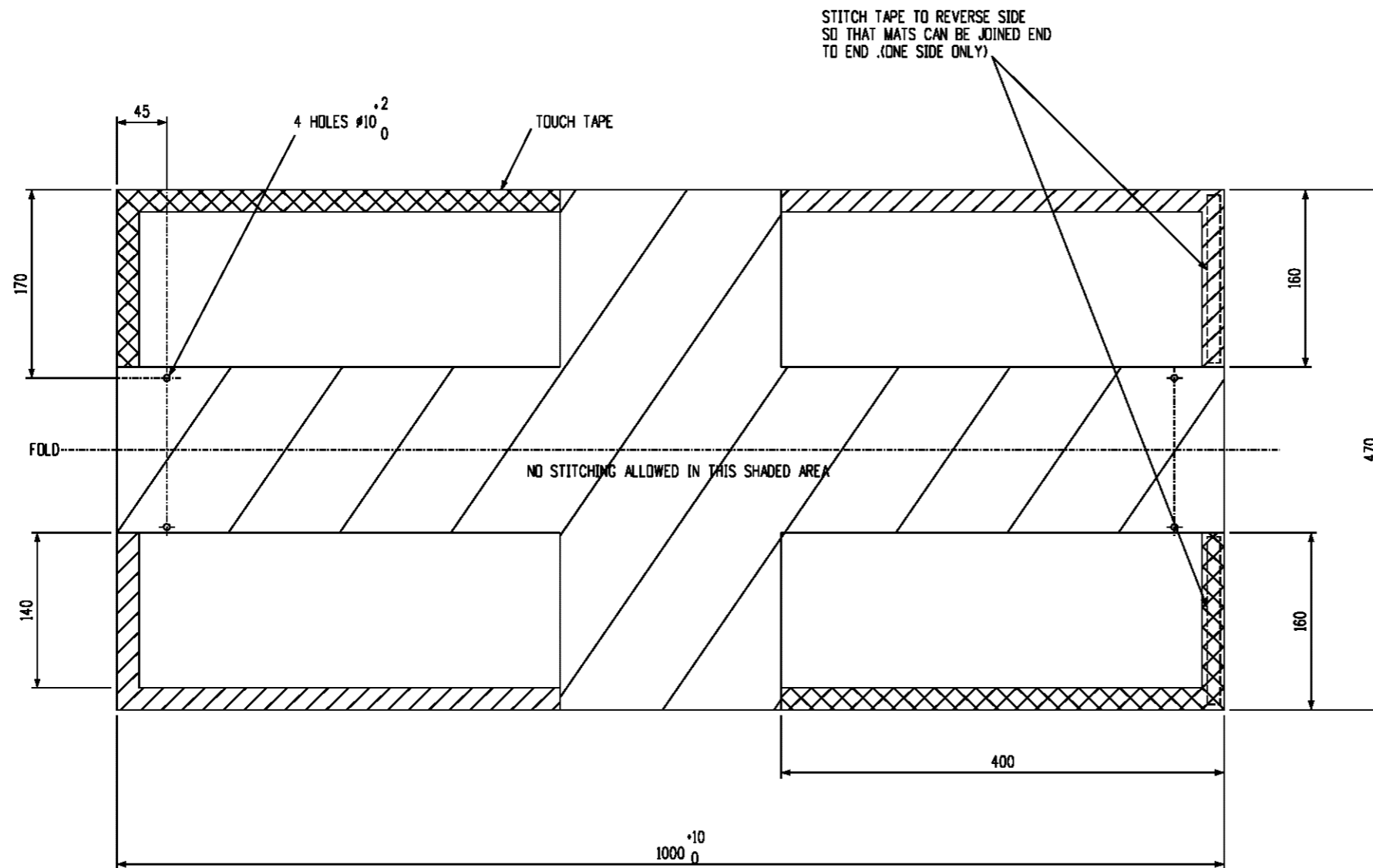
BARE L.V. CONDUCTOR INSULATING MAT (ITEM NUMBER:7641)
