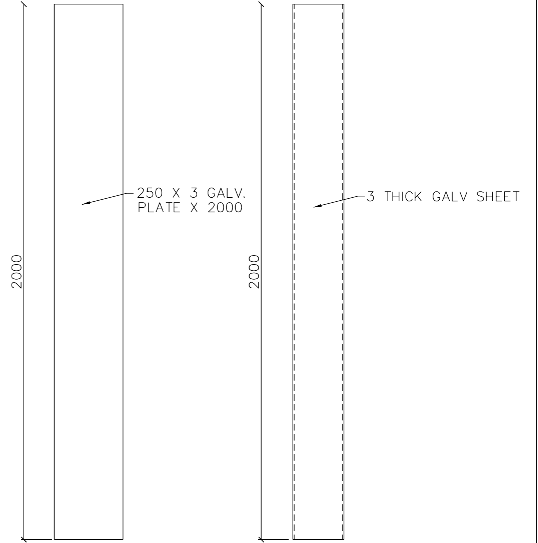
ITEM 4: CABLE PROTECTION PLUS BACKING PLATE FOR WEAK SIDE ALL POLES ITEM NUMBER: 504569
