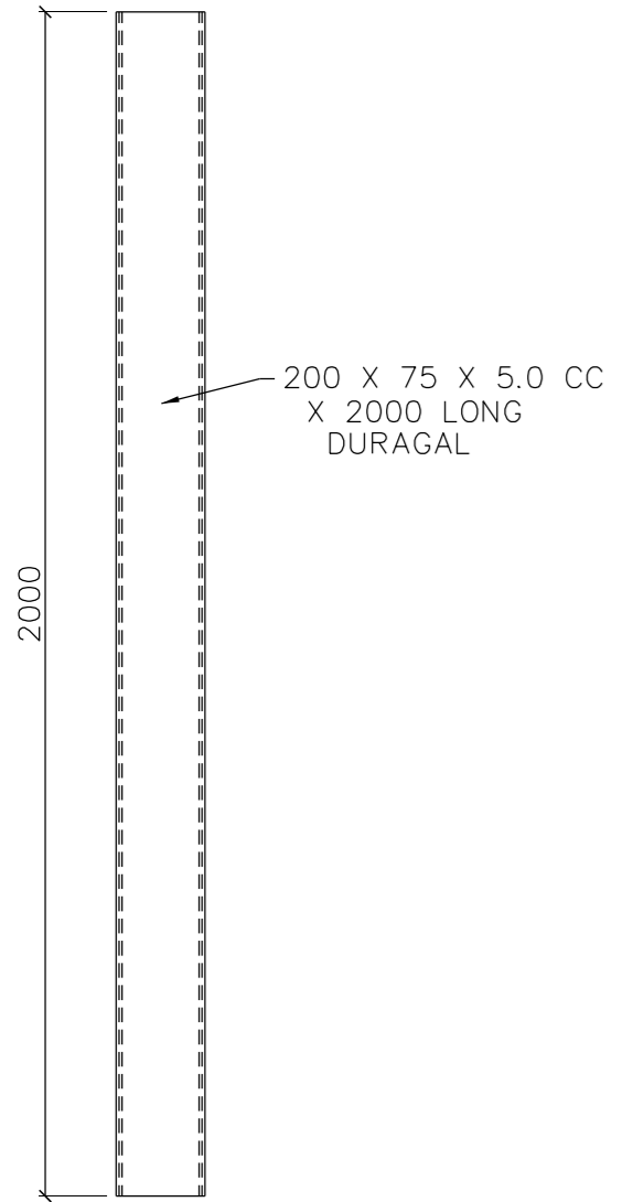
ITEM 1: TYPE B POLE STRONG SIDE ITEM NUMBER: 504549
