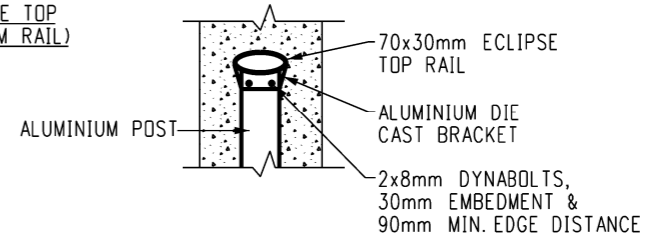
DETAIL-D TOP & BOTTOM RAIL END FIXING DETAILS
