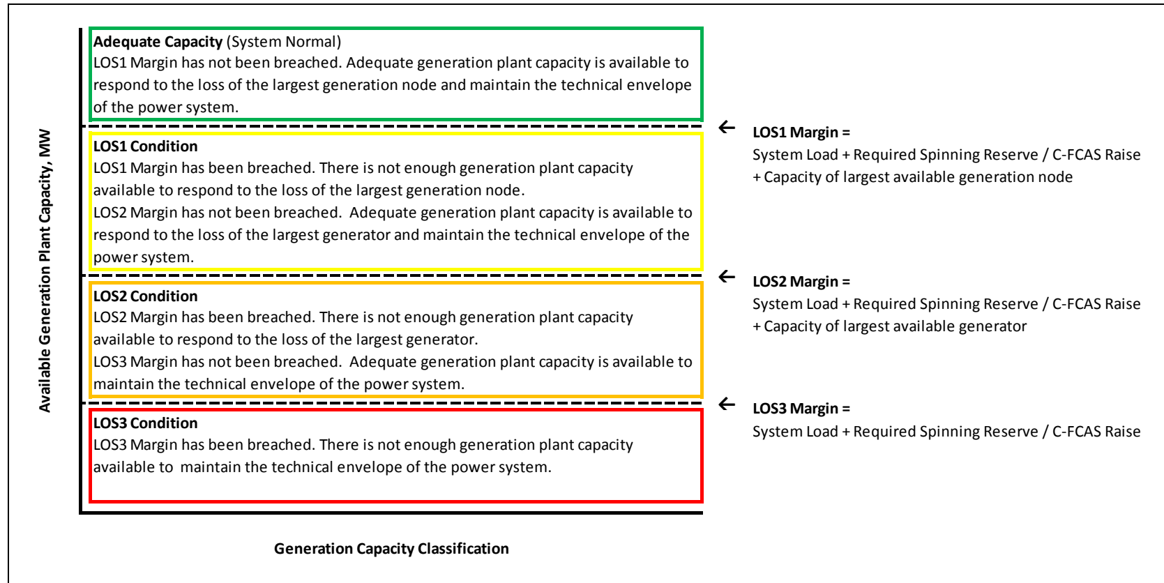
Figure 1: LOS Classification
