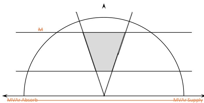
Figure 3 — Inverter-coupled Generation Unit reactive power capability
