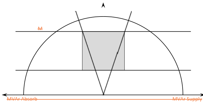
Figure 2—Induction Generation Unit reactive power capability
