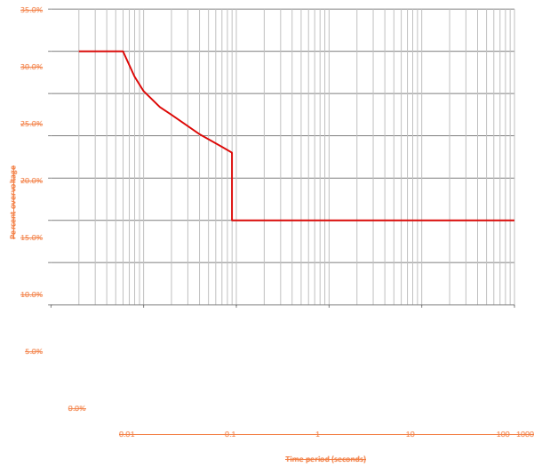
Figure 4 18 – Over voltage limit for contingency events
