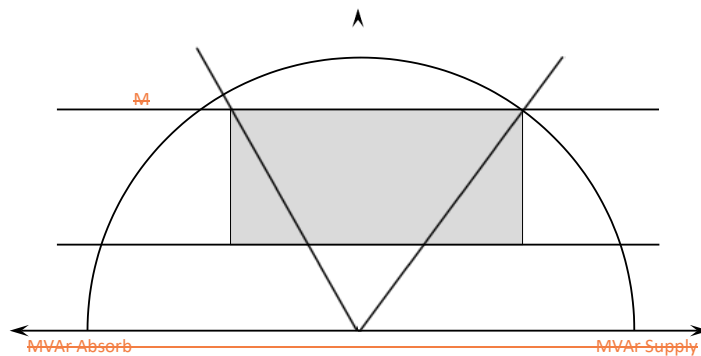
Figure 1 – Synchronous Generation Unit reactive power capability
