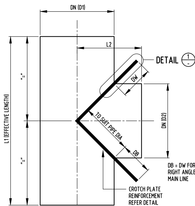
TEE JUNCTION - TYPE 1
