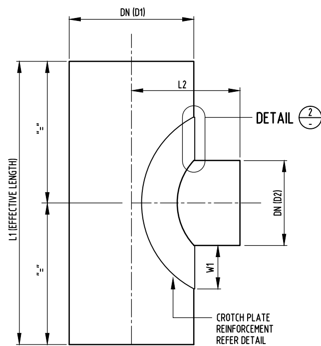
TEE JUNCTION - TYPE 2
