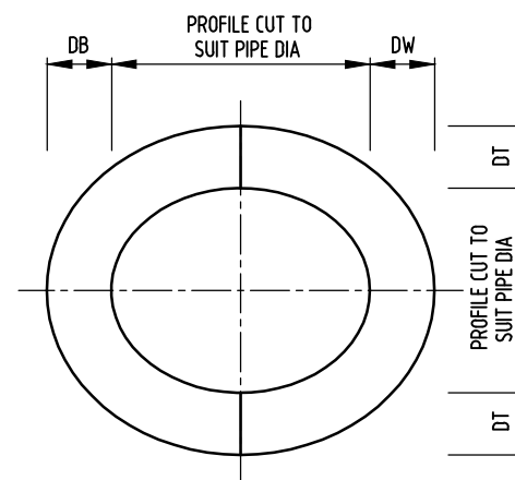
TEE JUNCTION CROTCH PLATE/ WRAPPER REINFORCEMENT
