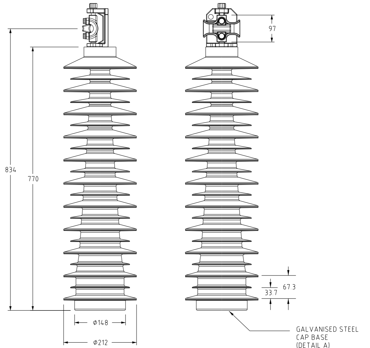
ITEM 2: HORIZONTAL LINE POST INSULATOR ITEM NUMBER: 503890
