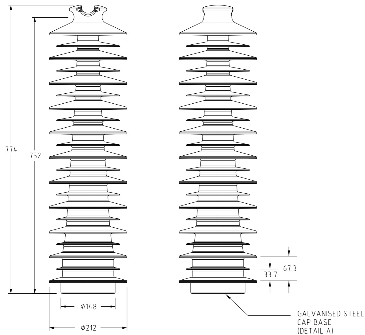
ITEM 1: VERTICAL LINE POST INSULATOR ITEM NUMBER: 503891
