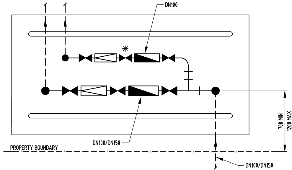
PLAN ORIENTATION OPTION 4
