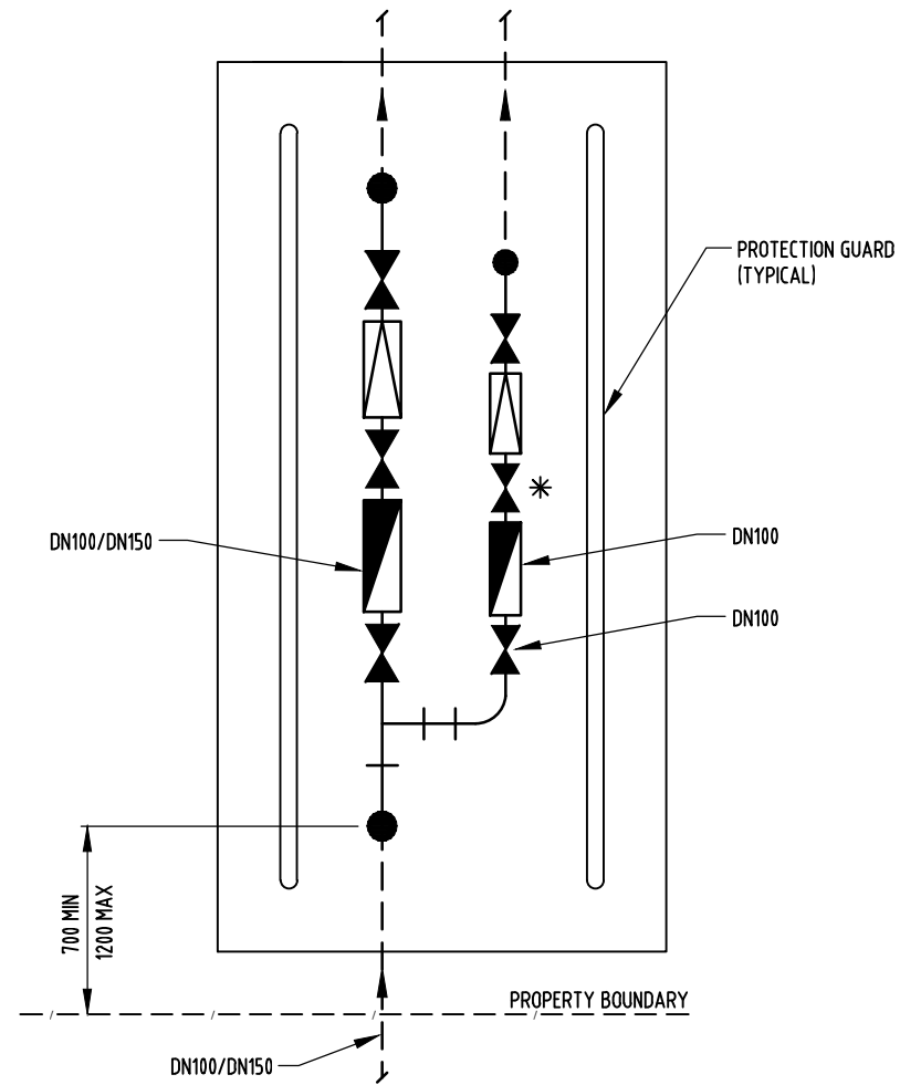
PLAN ORIENTATION OPTION 2
