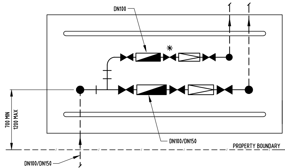
PLAN ORIENTATION OPTION 3
