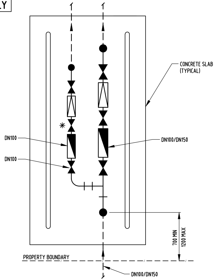
PLAN ORIENTATION OPTION 1
