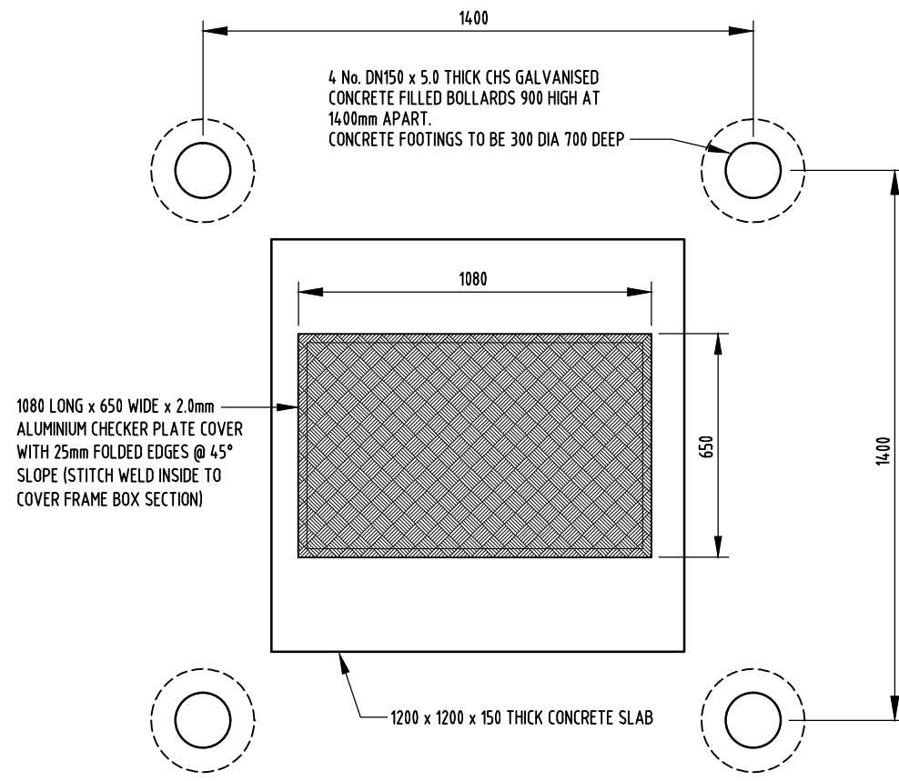
PLAN - TOP VIEW
