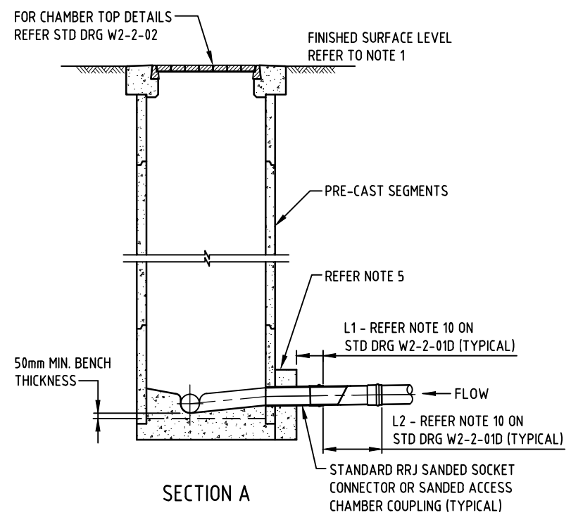
CIRCULAR ACCESS CHAMBER WITH RECTANGULAR COVER
