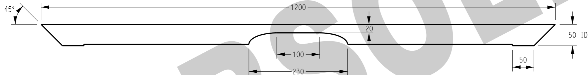
FRONT VIEW
