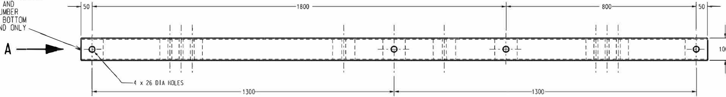
TOP VIEW
