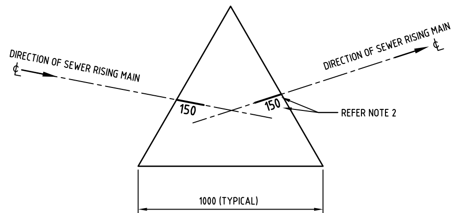
PLAN CONCRETE MARKER (FOR ABORIGINAL COMMUNITIES)
