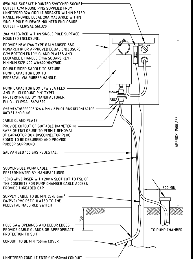
LOCKABLE ISOLATOR DETAIL NOT TO SCALE
