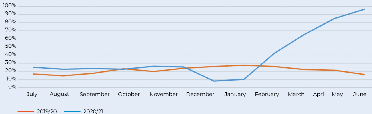
Figure 7 – Titjikala actual solar yield vs Atonometrics available yield
