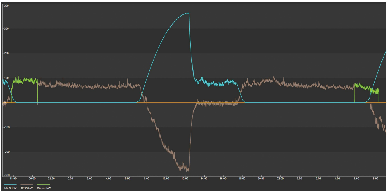
Figure 9 – Titjikala power station output 16-18 April 2021
