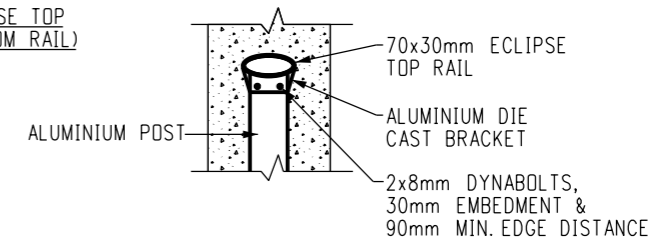
DETAIL-D TOP & BOTTOM RAIL END FIXING DETAILS
