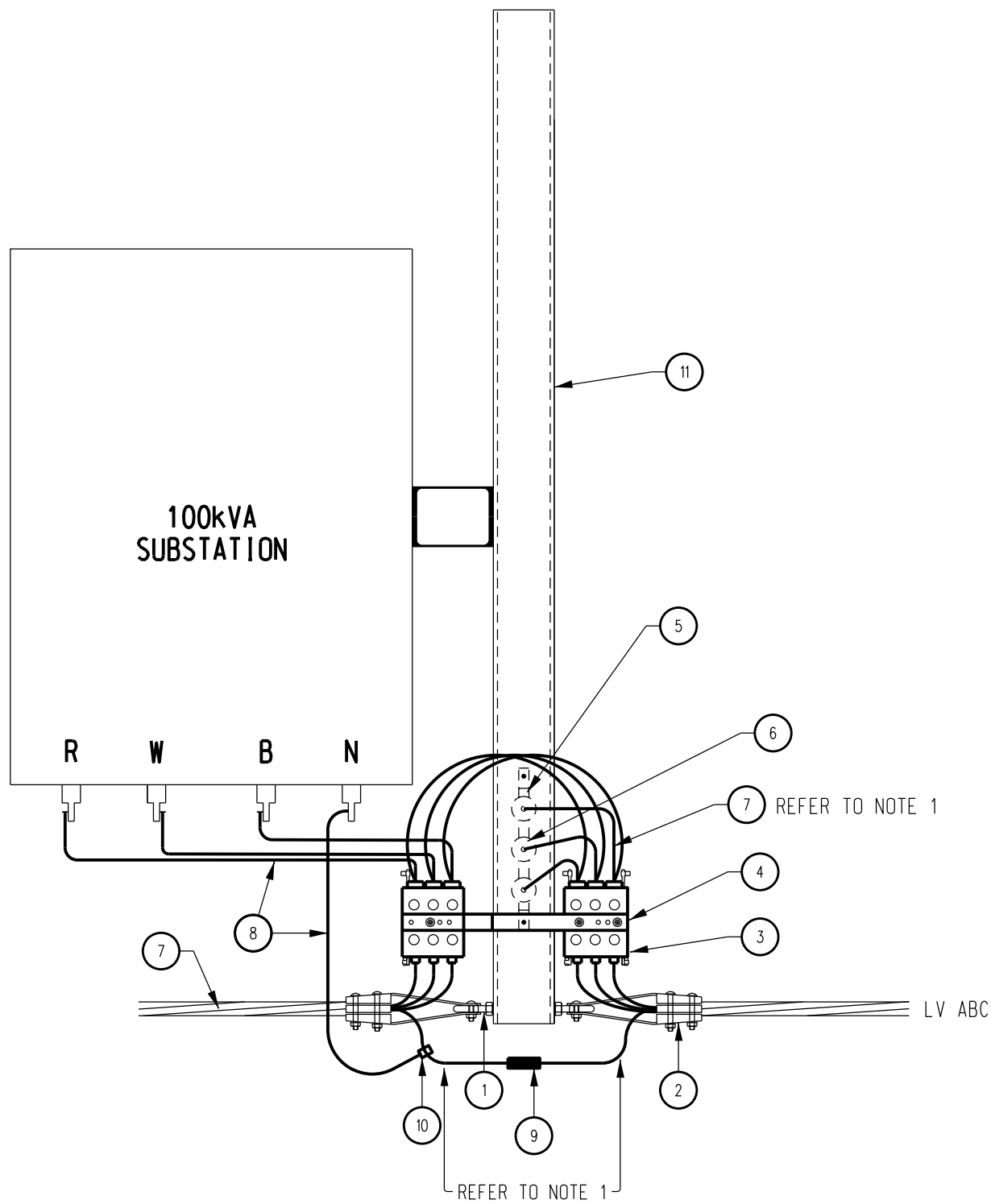
PLAN SCALE 1:15
