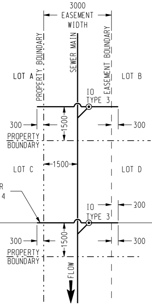
PLAN TYPE 3 CONNECTION LAYOUT FROM AN EASEMENT (NOT PREFERRED)
