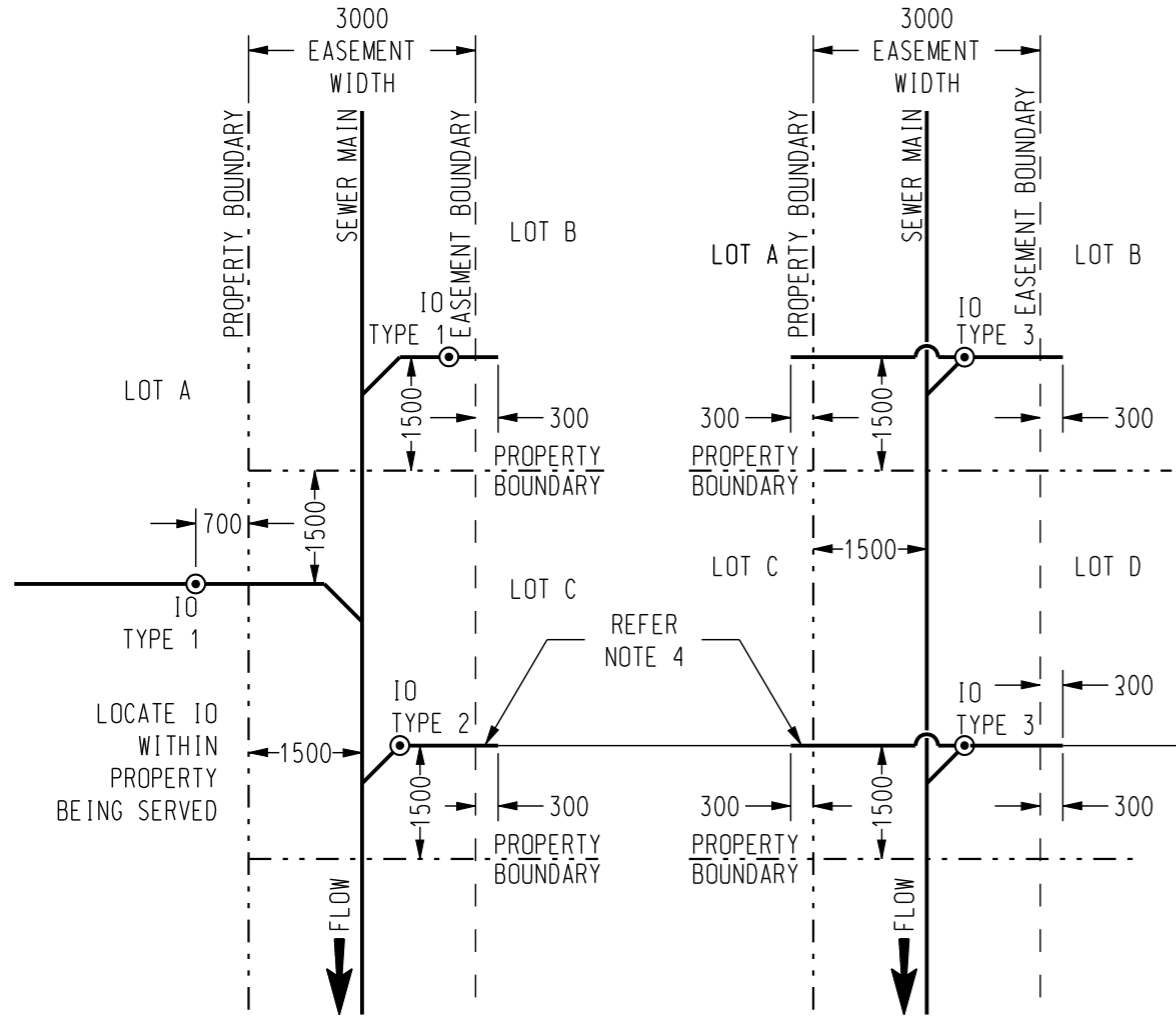
PLAN TYPE 1 & 2 CONNECTION LAYOUT FROM AN EASEMENT
