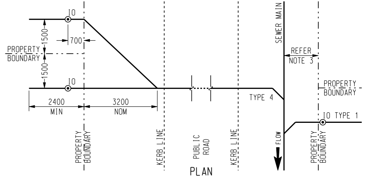
PLAN TYPE 4 CONNECTION LAYOUT
