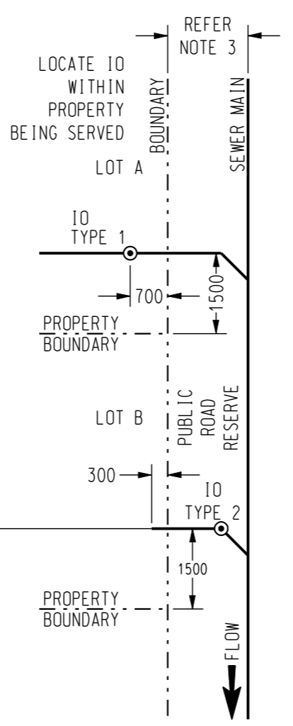
PLAN TYPE 1 & 2 CONNECTION LAYOUT FROM A ROAD RESERVE
