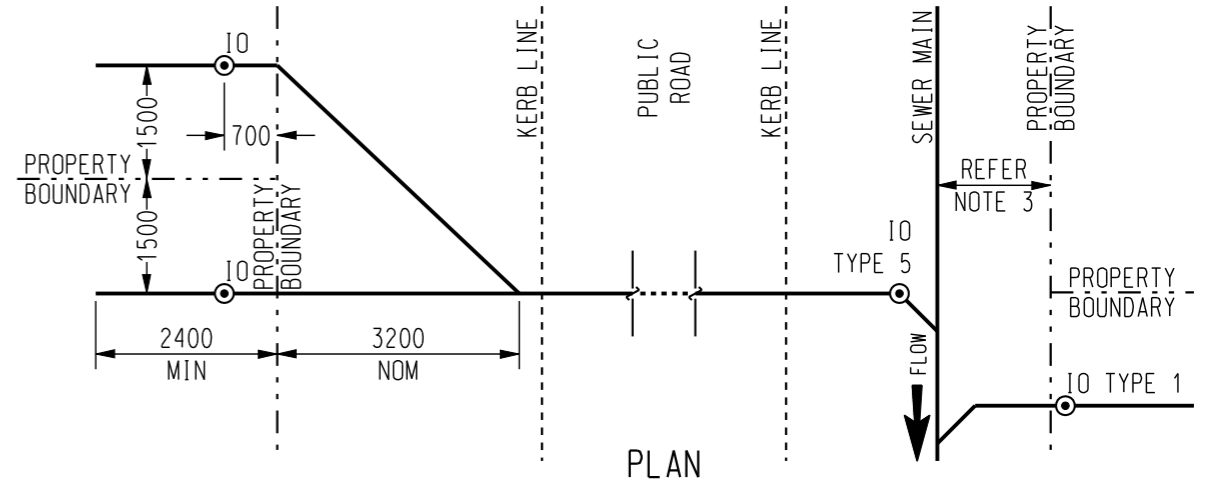
PLAN TYPE 5 CONNECTION LAYOUT
