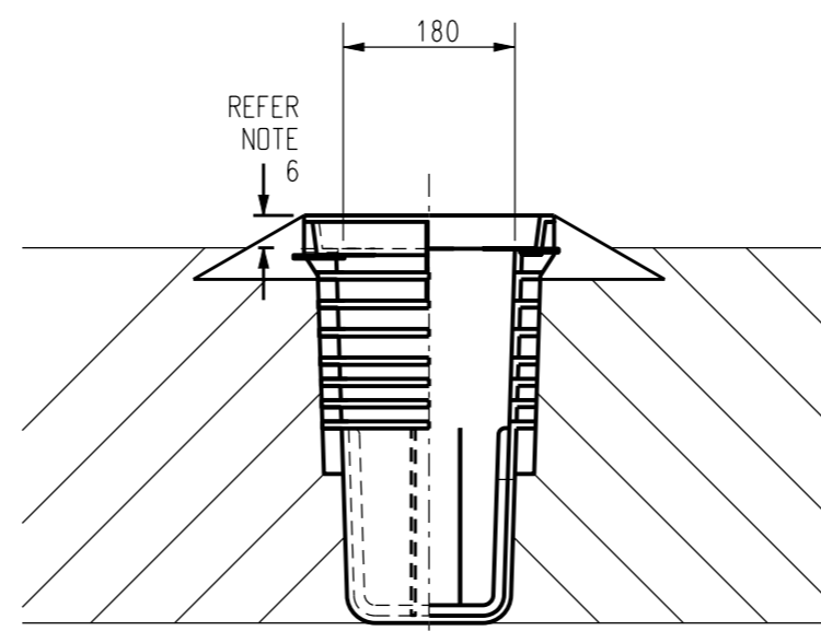
End Elevation/Section
