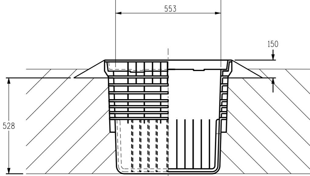
Elevation/Section
