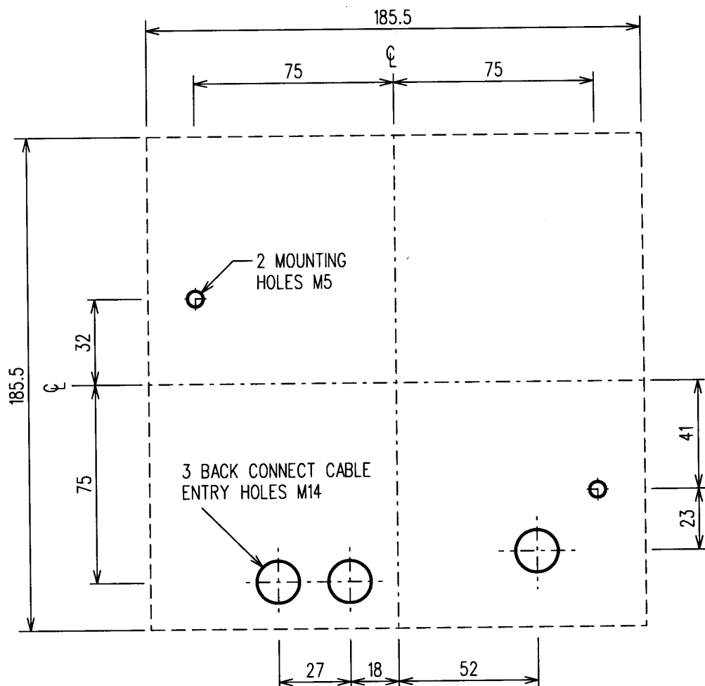
METER SOCKET - 3 JAW (EMAIL CAT. No. 828140)
