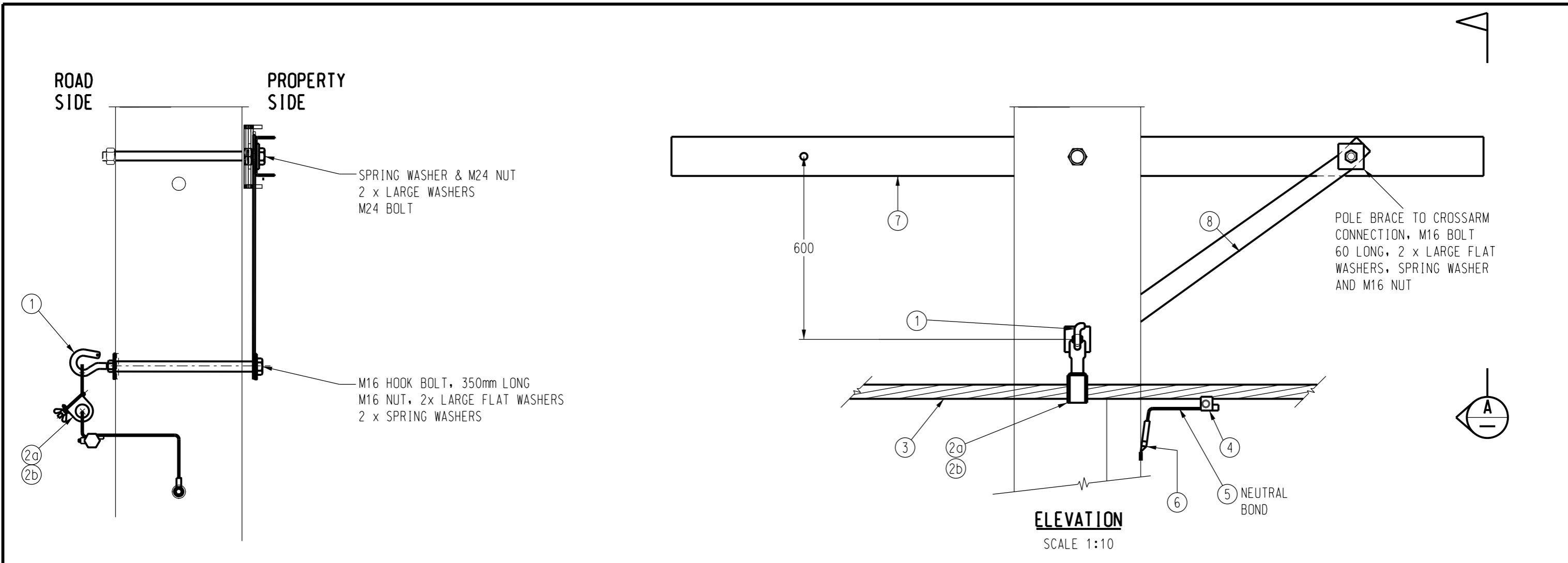
VIEW A SCALE 1:10
